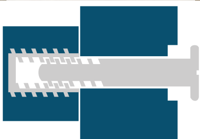
Angeles bolt & thread assembly
